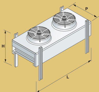
Horizontal installation
